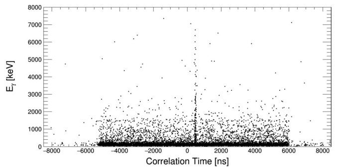
FIG. 3. Energies of \gamma rays detected in the TIGRESS array during a measurement of the ^{84}\text{Kr}(p, \gamma)^{85}\text{Rb} reaction as a function of TIGRESS-EMMA correlation time. A vertical cluster of counts indicates the observation of correlated primary and secondary \gamma rays, with energies approaching the p emission threshold in ^{85}\text{Rb} of 7 MeV, corresponding to ^{84}\text{Kr}(p, \gamma) events.
