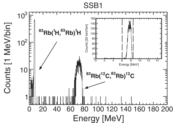
FIG. 1. Typical energy spectrum from one of the SSB detectors. The proton and carbon scattering peaks are labeled; the target constituents scattered by the 83 Rb and 83 Sr beam components are indistinguishable on the basis of energy and contribute to both of these peaks. The inset shows the same plot zoomed in on the proton scattering peak with selection cuts indicated by the vertical dashed lines.
