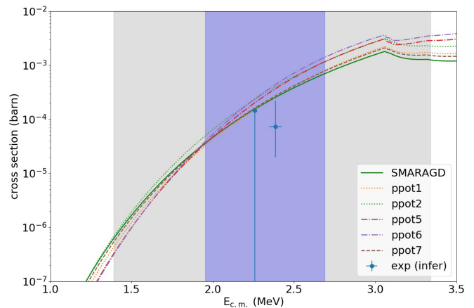
FIG. 8. Same as Fig. 7 but comparing the experimental data to SMARAGD calculations using various p + ^{83}\text{Rb} optical potentials (SMARAGD default [36,37], ppot1 [38], ppot2 [39], ppot5 [40], ppot6 [41], ppot7 [42]).
