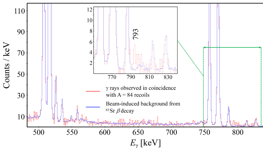
FIG. 5. \gamma rays observed in the eight TIGRESS detectors centered at 90^\circ with respect to the beam axis in coincidence with A = 84 recoils, following the ^{83}\text{Rb}(p, \gamma)^{84}\text{Sr} reaction. The inset shows a zoomed-in view of the same spectrum centered about the energy of the 793 keV transition.
