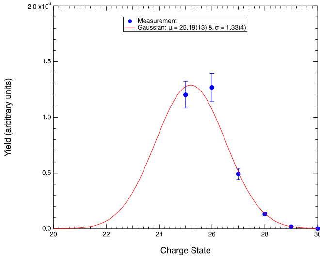
FIG. 2. Measured charge state distribution of ^{84}\text{Kr} incident at 2.7A MeV emerging from the 727 \mu\text{g cm}^{-2} polyethylene target. EMMA was set for a kinetic energy of 166 MeV during all of the yield measurements. The error bars represent systematic beam current uncertainties estimated to be \pm 10\% . Also shown are the results of a Gaussian fit.
