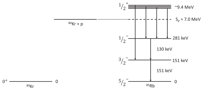
FIG. 4. Simplified energy level diagram of ^{85}\text{Rb} showing only levels relevant to this measurement of the ^{84}\text{Kr}(p, \gamma)^{85}\text{Rb} reaction. The states initially populated via s -wave capture are shown schematically about 2.4 MeV above the proton separation energy S_p .
