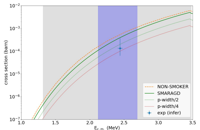
FIG. 9. Same as Fig. 7 but for the ^{84}\text{Kr}(p, \gamma)^{85}\text{Rb} reaction.
