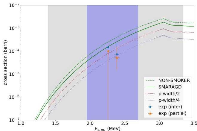
FIG. 7. Cross section of the ^{83}\text{Rb}(p, \gamma)^{84}\text{Sr} reaction from experiment (shown are the partial cross section for populating the 2_1^+ state and the inferred total cross section with 90% CL error bars) compared to statistical model predictions of the total cross sections with the NON-SMOKER [15] and SMARAGD [34] codes. The wider, lightly shaded region indicates the approximate location of the relevant energy window [16] for the ^{83}\text{Rb}(p, \gamma)^{84}\text{Sr} reaction in ccSNe ( 2 \text{ GK} < T < 3.5 \text{ GK} ). The narrower, darkly shaded region indicates the range of relative kinetic energies covered in the measurement of the E_{c.m.} = 2.386 MeV data point. The measured and inferred points at E_{c.m.} = 2.26 MeV are 90% CL upper limits. Also shown are SMARAGD calculations with the default proton width divided by two and four, respectively.
